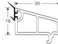
NAME: 30 glazing bead CODE: 30YX WEIGHT(KG/M): 0.275 LENGTH: 5.9m KG/PIECE: 1.65 PCS/BAG: 20 THICKNESS: 1.6 a
