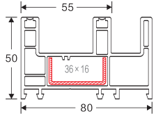
NAME: 80 sliding frame H3 CODE: TL80KH3 WEIGHT(KG/M): 1.317 LENGTH: 5.9m PCS/BAG: 6 THICKNESS: 2.2 aeel
