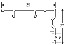
NAME: 80 sliding sash cover CODE: 80FG WEIGHT(KG/M): 0.18 LENGTH: 5.9m PCS/BAG: 30 THICKNESS: ae
