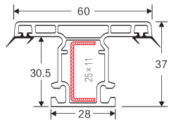
NAME: 80 sash mullion CODE: 80S2T WEIGHT(KG/M): 0.67 LENGTH: 5.9m KG/PIECE: 4.02 PCS/BAG: 8 THICKNESS: 1.6 a
