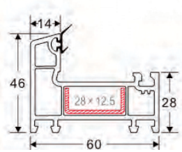
NAME: 60 small frame CODE: 60XK WEIGHT(KG/M): 0.88 LENGTH: 5.9m PCS/BAG: 6 THICKNESS: 2.2
