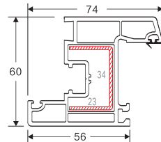
NAME: 60 in-swing window sash A CODE: 60NKCSA WEIGHT(KG/M): 1.20 LENGTH: 5.9m PCS/BAG: 6 THICKNESS: 2.2 a c e e h i
