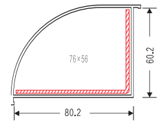
NAME: 80-60 bay corner adaptor CODE: 80Z60ZJ WEIGHT(KG/M): 0.78 LENGTH: 5.9m PCS/BAG: 4 THICKNESS: 1.8 a
