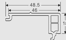
NAME: Shutter glazing bead CODE: BYCZYYT WEIGHT(KG/M): 0.26 LENGTH: 5.9m PCS/BAG: 20 THICKNESS: a
