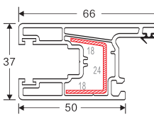
NAME: 80 big sliding sash B CODE: 80TLDSB WEIGHT(KG/M): 0.91 LENGTH: 5.9m PCS/BAG: 8 THICKNESS: 2.0 ae
