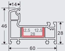
NAME: 60 small frame CODE: 60XK WEIGHT(KG/M): 0.85 LENGTH: 5.9m PCS/BAG: 6 THICKNESS: 2.2
