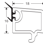
NAME: 18 glazing bead CODE: 18YX WEIGHT(KG/M): 0.22 LENGTH: 5.9m KG/PIECE: 1.32 PCS/BAG: 30 THICKNESS: Glass Thickness: 22±0.5mm a
