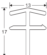
NAME: Round bead CODE: PT WEIGHT(KG/M): 0.092 LENGTH: 5.9m PCS/BAG: 50 THICKNESS: a
