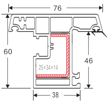
NAME: 60 out-swing window sash 2 CODE: 60WKCS2 WEIGHT(KG/M): 1.21 LENGTH: 5.9m PCS/BAG: 6 THICKNESS: 2.2 a c e e h i
