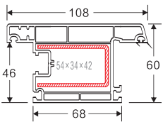
NAME: 60 out-swing door sash 2 CODE: 60WKMS2 WEIGHT(KG/M): 1.65 LENGTH: 5.9m PCS/BAG: 4 THICKNESS: 2.2 a i
