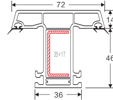
NAME: 60 mullion D CODE: 60ZTD WEIGHT(KG/M): 1.149 LENGTH: 5.9m PCS/BAG: 6 THICKNESS: 2.2 a b c d e f g h i
