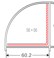
NAME: 60 bay corner adaptor 2 CODE: 60ZJ2 WEIGHT(KG/M): 0.71 LENGTH: 5.9m PCS/BAG: 4 THICKNESS: 1.8 a
