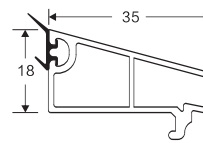
NAME: 60 single glazing bead A CODE: 60DYA WEIGHT(KG/M): 0.317 LENGTH: 5.9m PCS/BAG: 20 THICKNESS: 1.6 a
