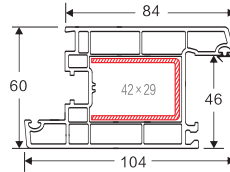
NAME: 60 in-swing door sash 2 CODE: 60NKMS2 WEIGHT(KG/M): 1.517 LENGTH: 5.9m PCS/BAG: 4 THICKNESS: 2.2 a i
