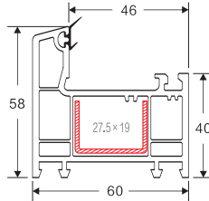
NAME: 60 frame D CODE: 60PKD WEIGHT(KG/M): 1.042 LENGTH: 5.9m PCS/BAG: 6 THICKNESS: 2.2 a b c d e f g h i
