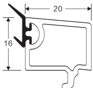
NAME: 80 glazing bead B CODE: 80DYB WEIGHT(KG/M): 0.22 LENGTH: 5.9m PCS/BAG: 30 THICKNESS: a
