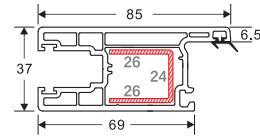
NAME: 80 sliding door sash CODE: 80TLMS WEIGHT(KG/M): 1.3 LENGTH: 5.8-6.0m PCS/BAG: 8 THICKNESS: 2.5
