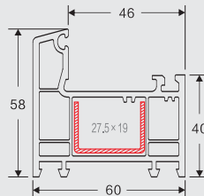
NAME: 60 frame D CODE: 60PKD WEIGHT(KG/M): 1.012 LENGTH: 5.9m PCS/BAG: 6 THICKNESS: 2.2 a b c d e f g h i
