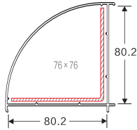
NAME: 80 bay corner adaptor 1 CODE: 80ZJ1 WEIGHT(KG/M): 0.78 LENGTH: 5.9m PCS/BAG: 4 THICKNESS: 1.6 a
